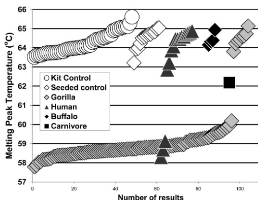
FIGURE 1. Spectrum of melting peak temperatures for R.A.P.I.D. (Idaho Technology Inc., Salt Lake City, Utah, USA) replicates from different types of specimens.
